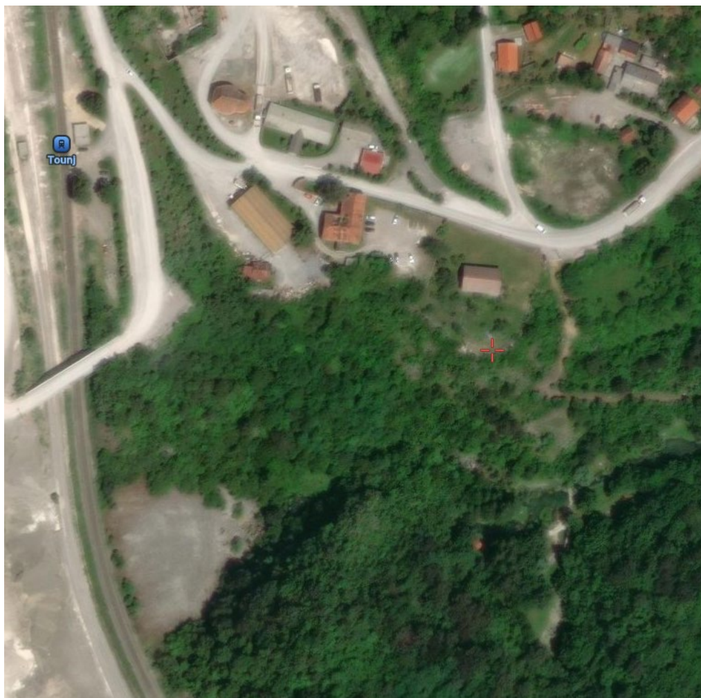
F.41. Tounj satelitska karta 2025. ( https://satellites.pro/Tounj_map#45.249730,15.322768,18 )
